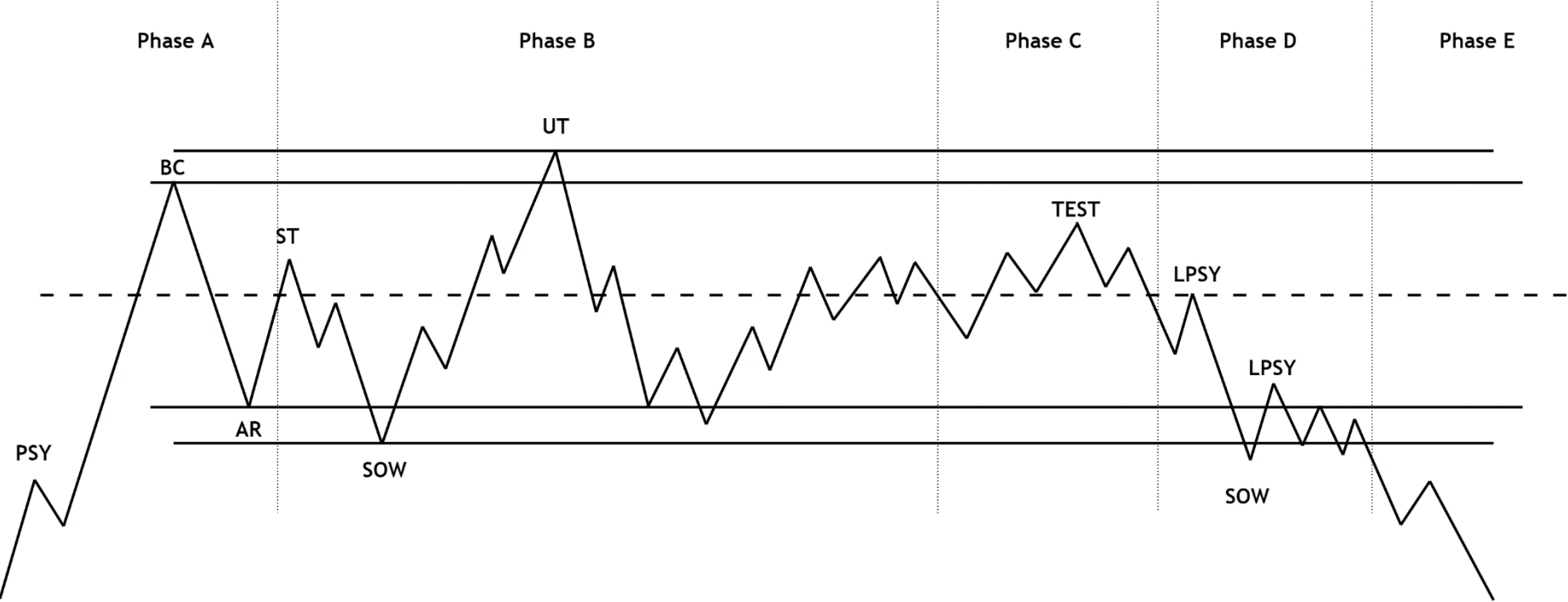
Distribution Schematic #2
