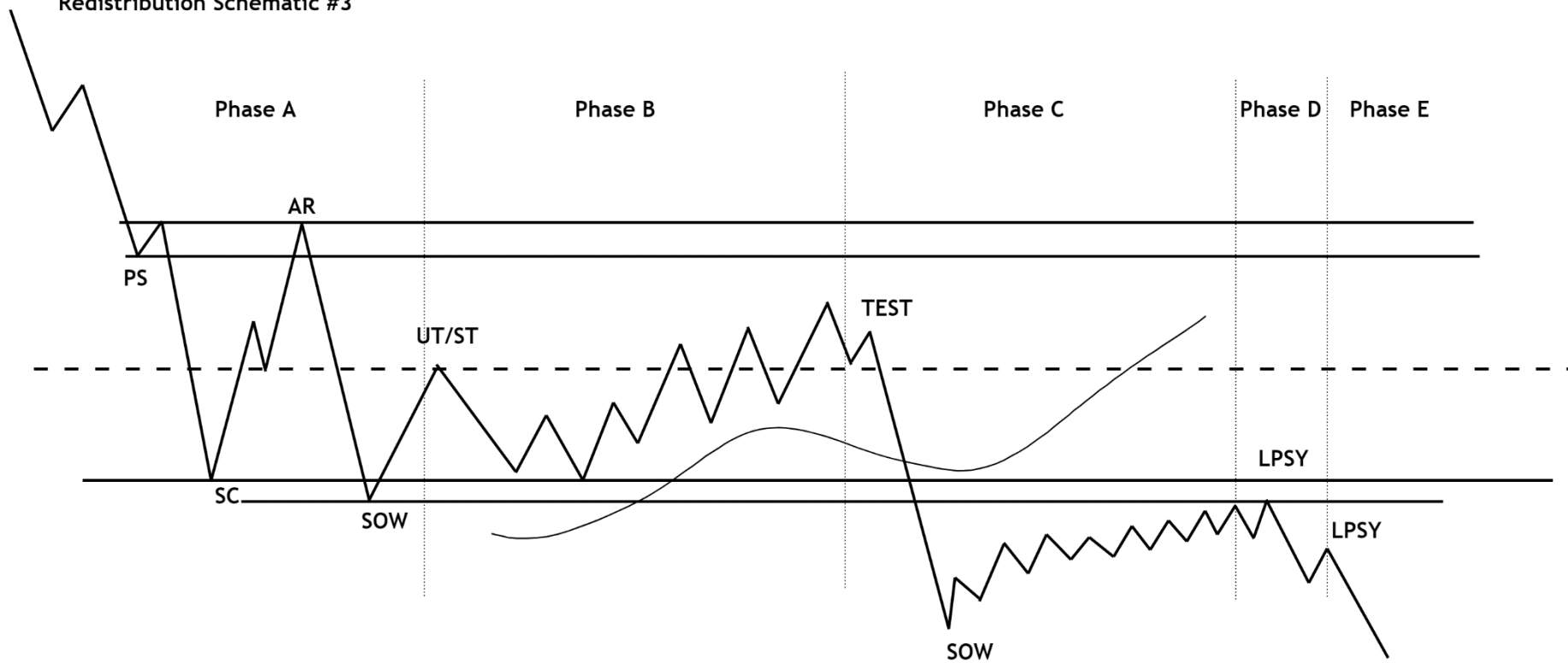
Redistribution Schematic #3
