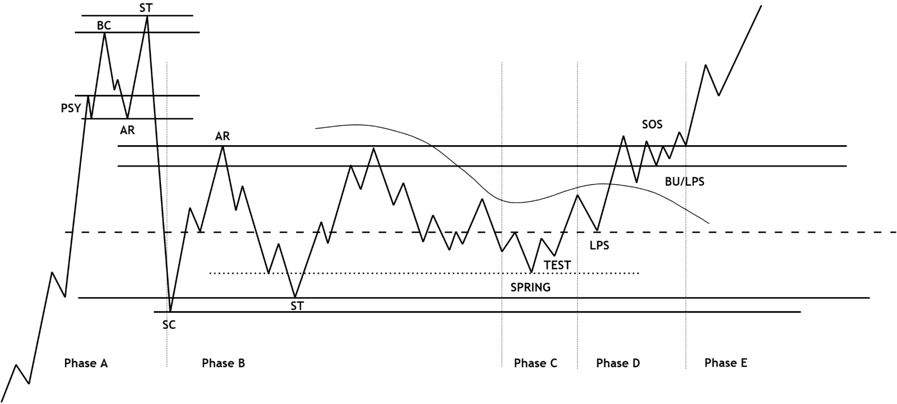
Reaccumulation Schematic #4
