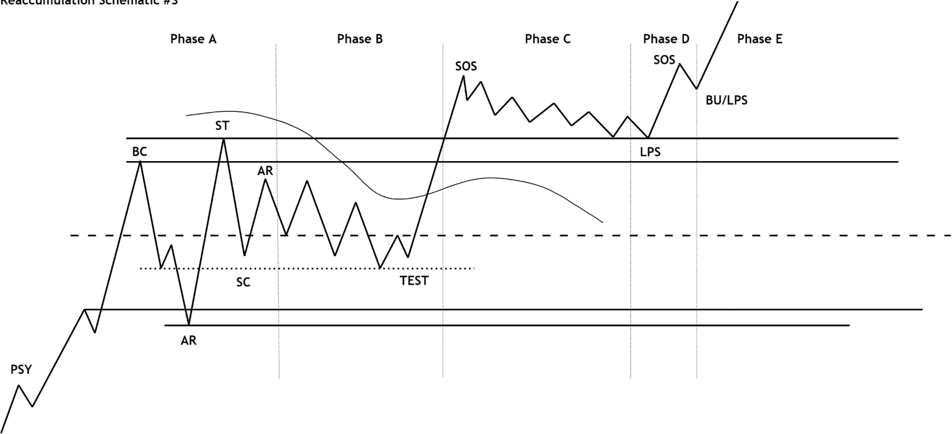
Reaccumulation Schematic #3
