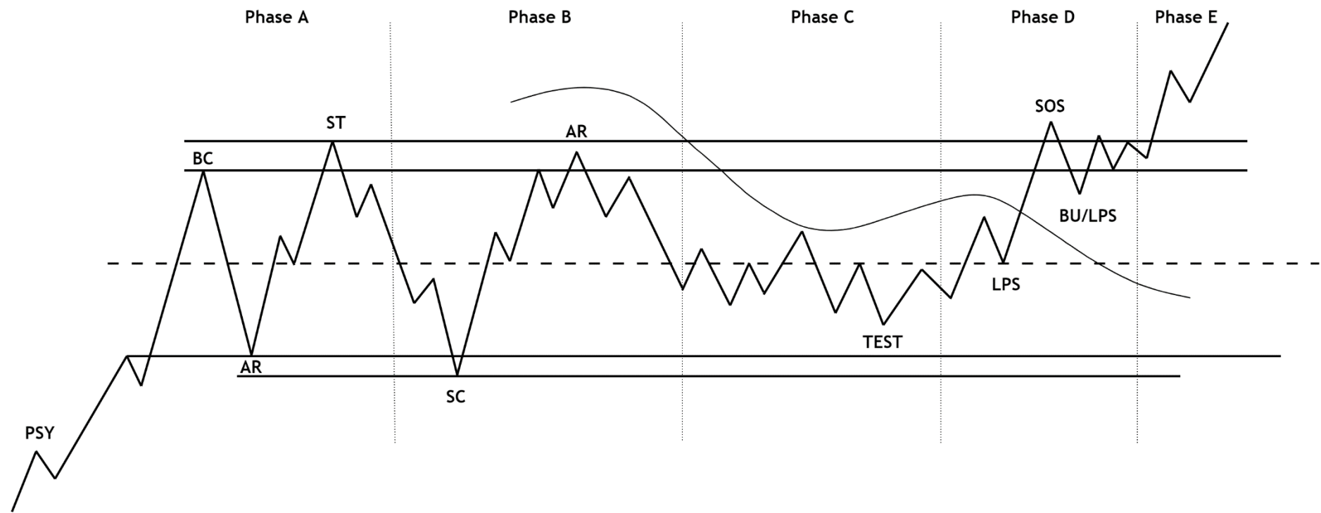
Reaccumulation Schematic #2
