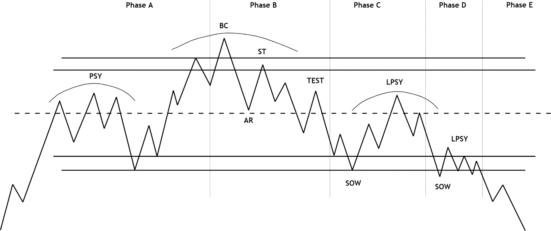
Distribution Schematic #3
