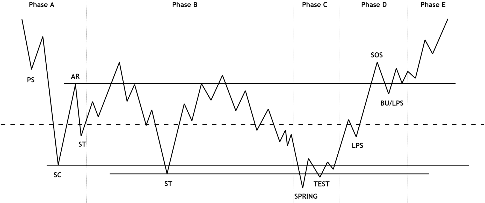
Accumulation Schematic #1
