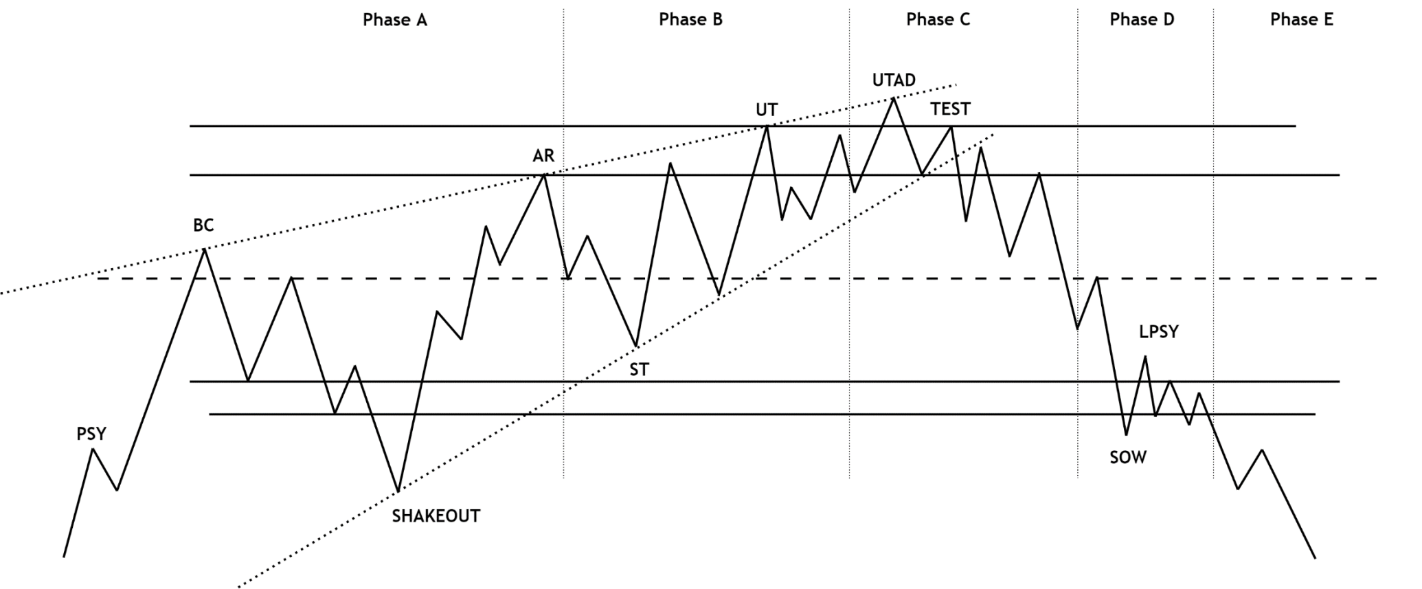
Distribution Schematic #4
