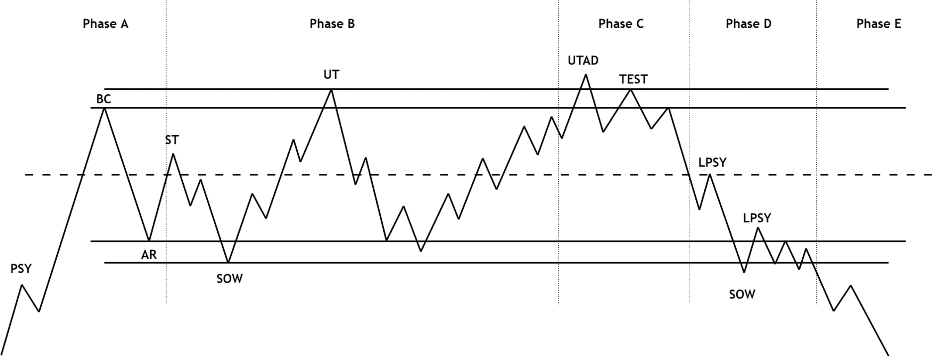
Distribution Schematic #1
