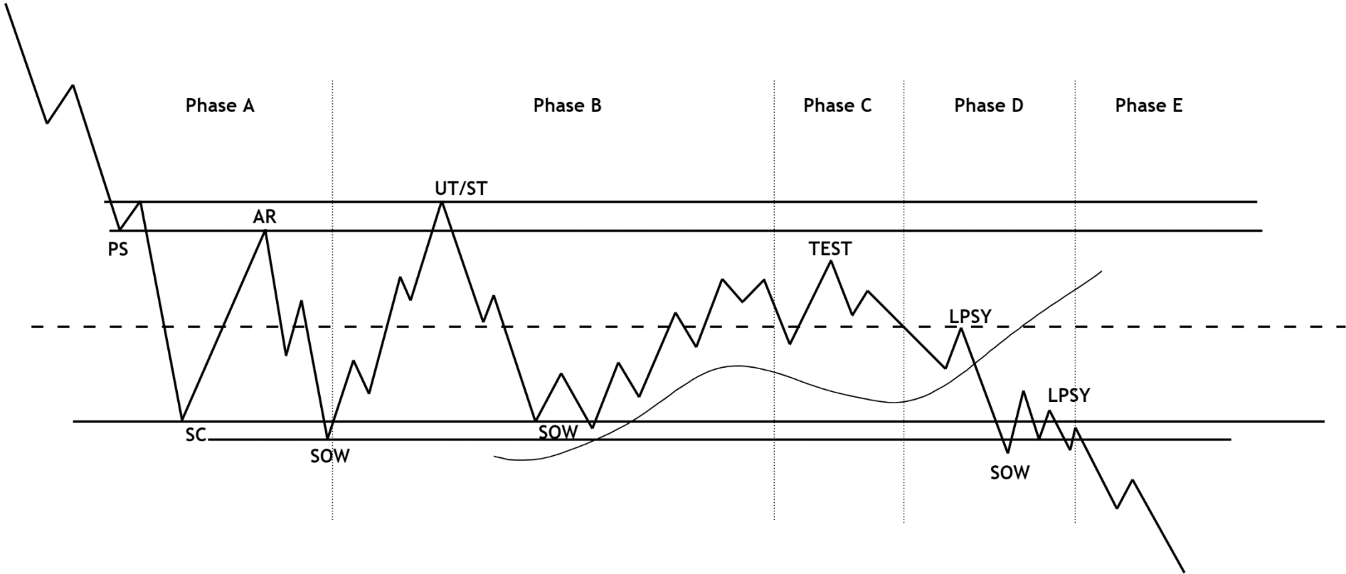
Redistribution Schematic #2
