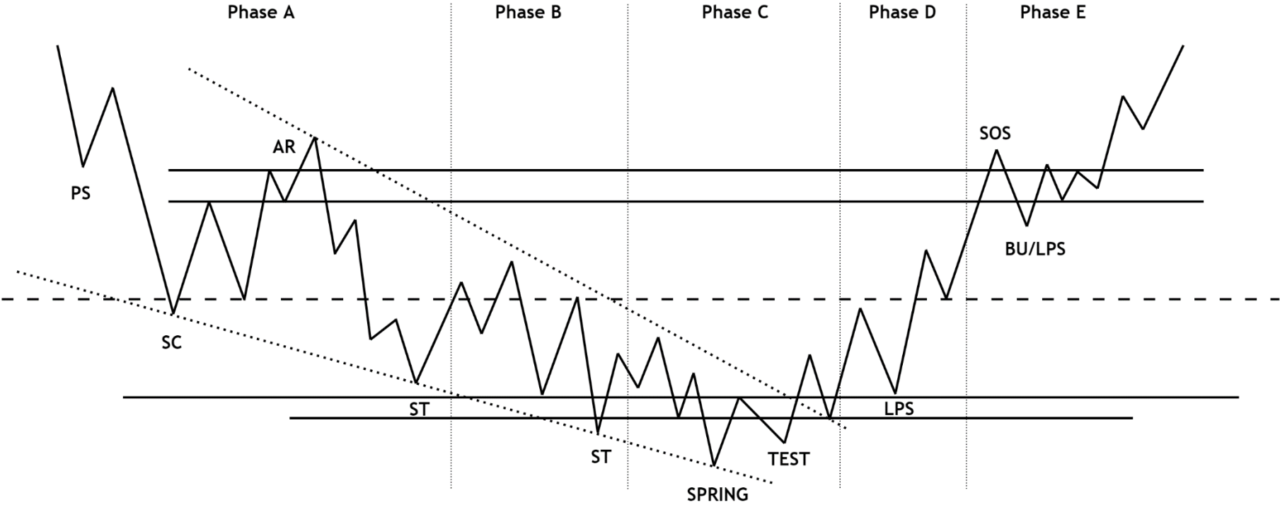
Accumulation Schematic #4
